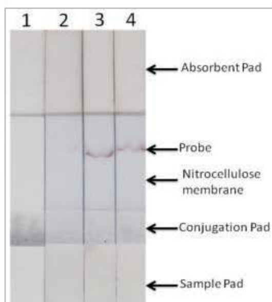
Detection of oxytetracycline by lateral flow method
